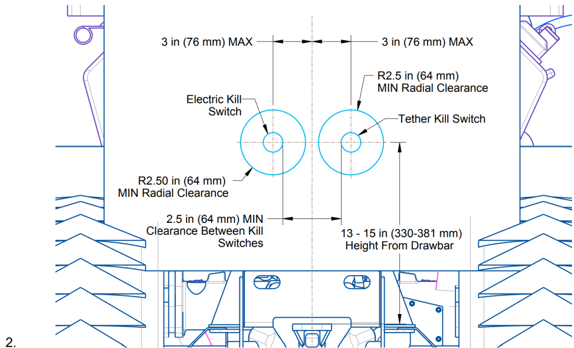
Figure 7 - Kill Switch Detail
