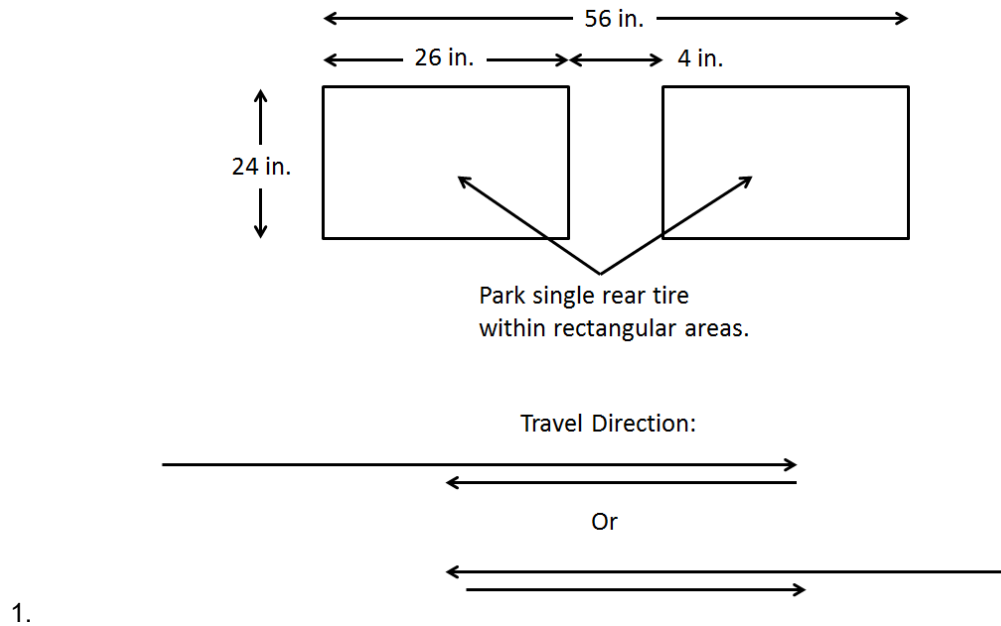
Figure 13 - Controllability Test Layout
